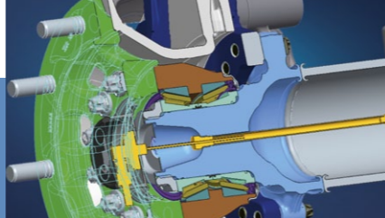
Tyre pressure monitoring with rim sensor and automatic refilling function.
